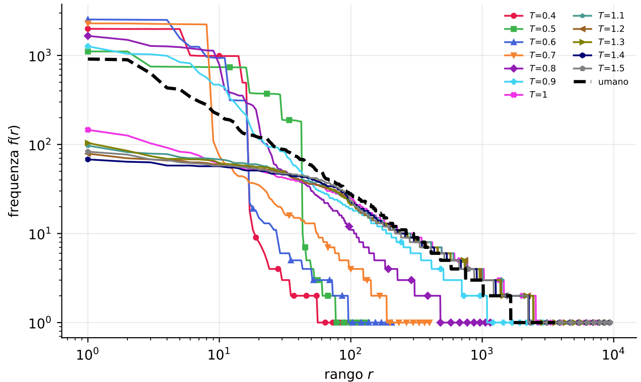
Rango-frequenza — Qwen2.5-1.5B (cfr. [L] Fig. 2A)
