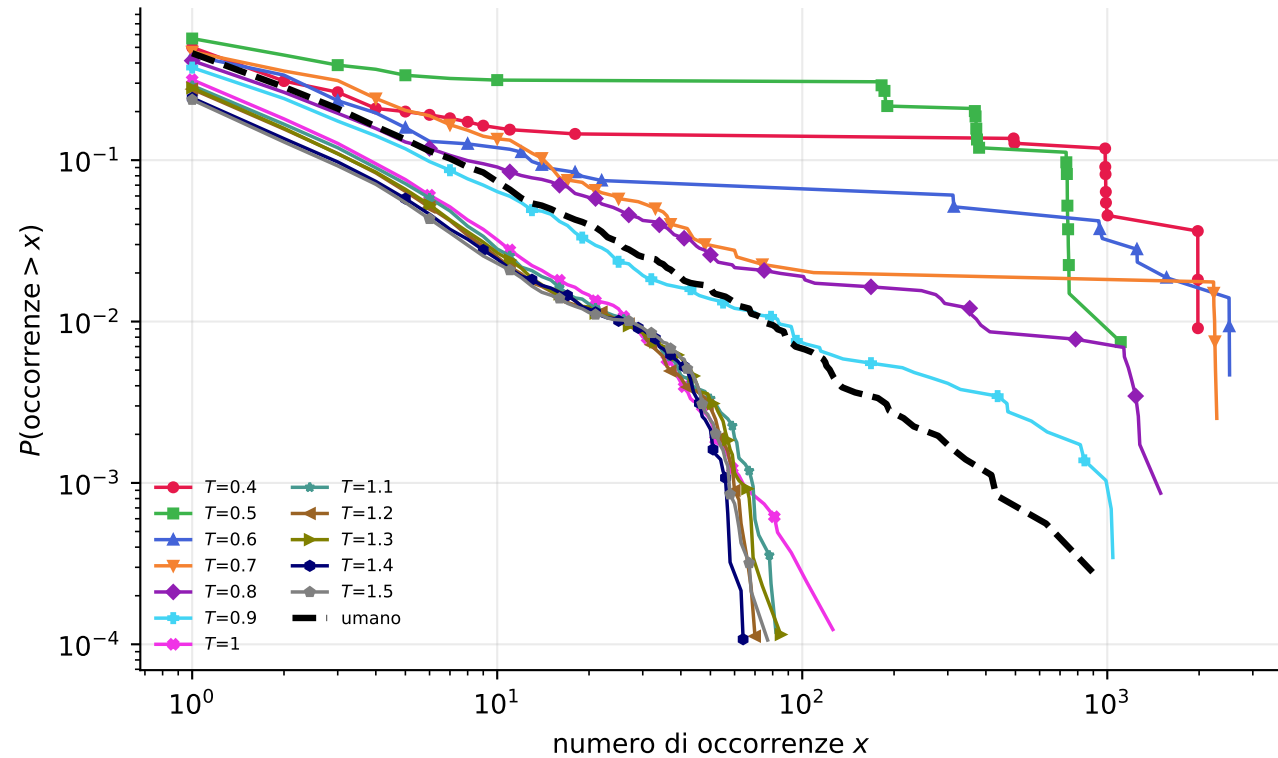
Istogramma cumulativo — Qwen2.5-1.5B (cfr. [Z] Fig. 6)
